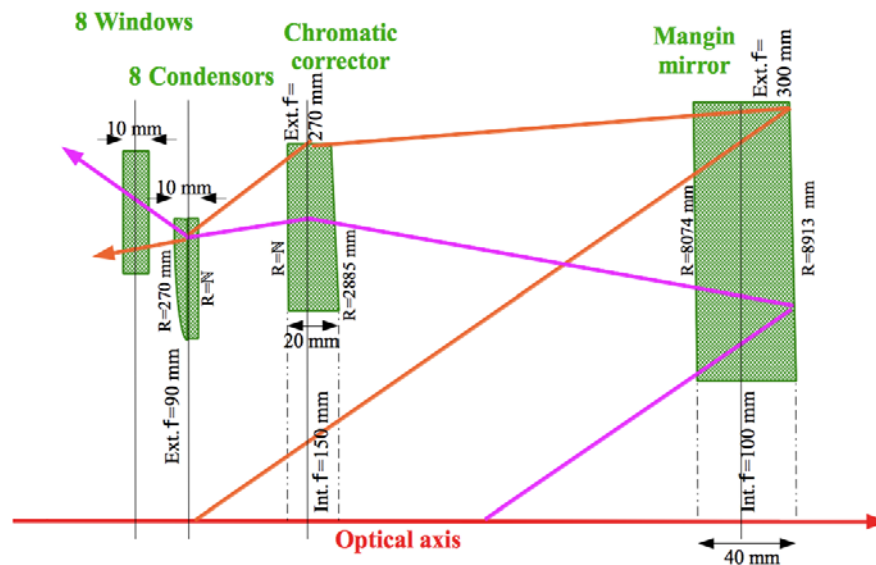
Figure 2: Schematic layout of the optical elements and the light path.
