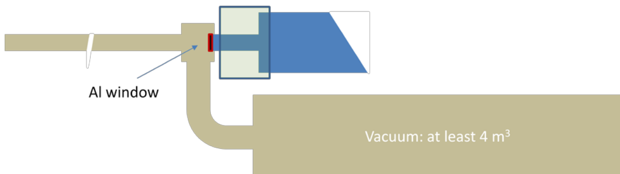
Figure 5: Conceptual drawing of the retention vacuum volume attached to the upstream end of the CEDAR (in blue). The aluminum window on the upstream side has thickness of 150\ \mu\text{m} , the downstream window has a thickness of 200\ \mu\text{m} .
