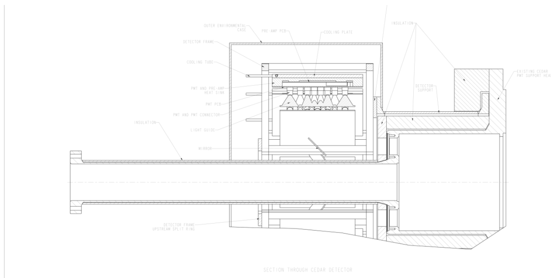
Figure 6 : Cross-sectional Layout of the Support Structure and Nitrogen Enclosure
