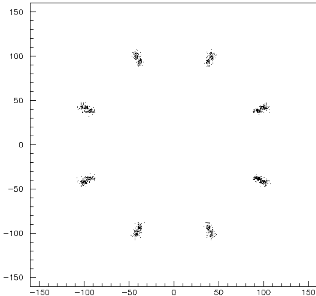
Figure 8: Distribution of photons on the 8 quartz windows at the exit of the CEDAR
