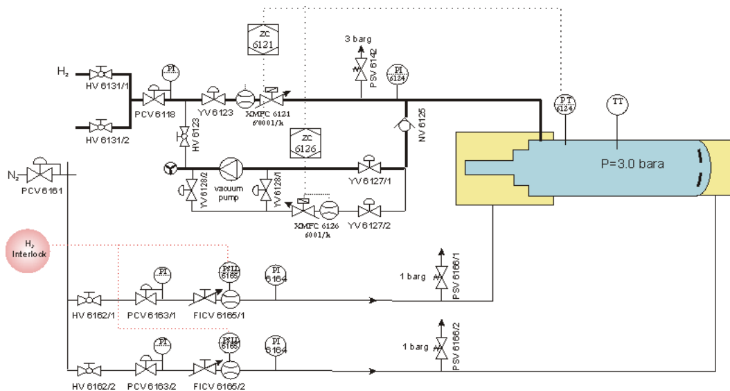
Figure 7: Layout of the CEDAR gas system (blue = CEDAR radiator volume, yellow = envelope volumes)
