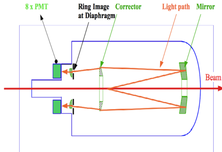
Figure 1 Schematic layout of the Standard West-Area CEDAR.
