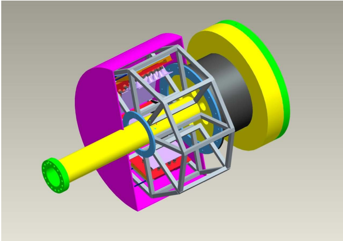
Figure 4: Conceptual Design of the Support Structure and Nitrogen Enclosure.
