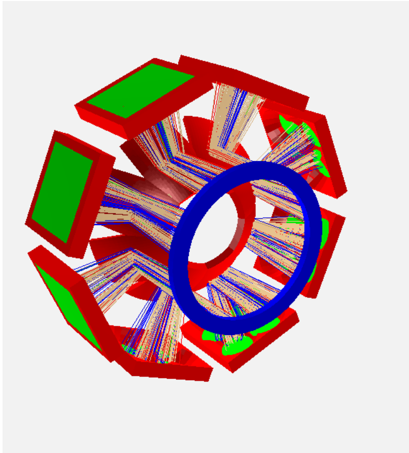
Figure 3: The Simulation of 100 events in the CEDAR nose cone. The ray tracing of the photons from (right to left) the quartz window (blue), the ellipsoidal mirrors (red), the light collection cones (red) and photodetector plane (green) is illustrated. The optical components are schematic and do not reflect a final geometrical arrangement. The photons are shown in fawn for those that are detected directly and blue if detected after reflection from the cone. Photons that are lost at reflection in the cone are shown in green whilst those photons lost by reflection at the PMT window are indicated in red.
